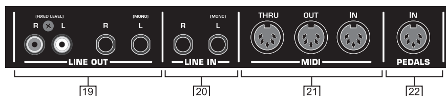
Fig. 4.2 Connectors of the EG2080
